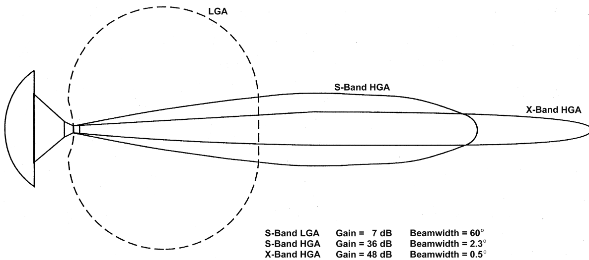
Fig. 3-2. Voyager S-XA patterns and beamwidths.
